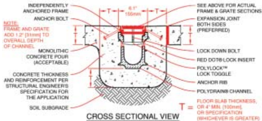
Cross-Sectional View Channel with Frame and Grate
